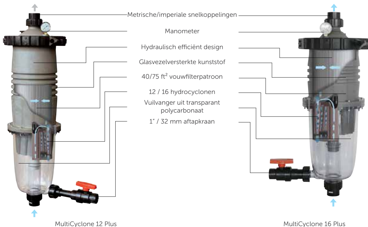
MultiCyclone 12 Plus
